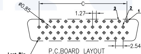
P.C. BOARD LAYOUT (68,100Pin) R2 Type / 反脚位
