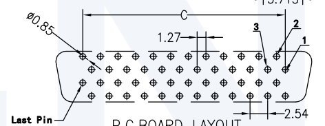
P.C. BOARD LAYOUT (68,100Pin) R1 Type / 正脚位
