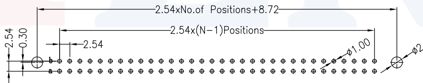
Recommended P.C.B Layout(Top Side) (PCB BOARD TOLERANCE±0.05)
