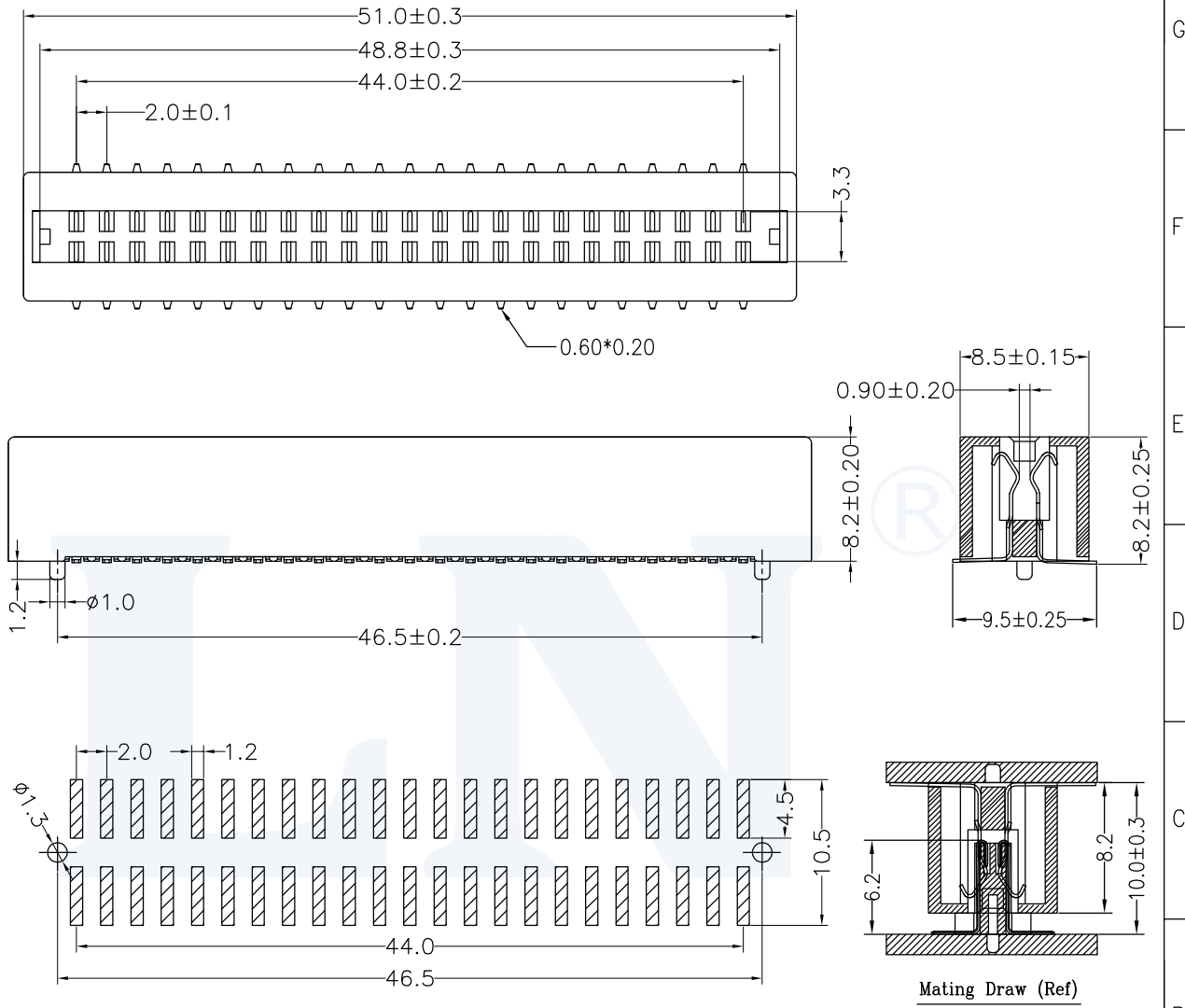
Recommended P.C.B Layout(Top Side)
