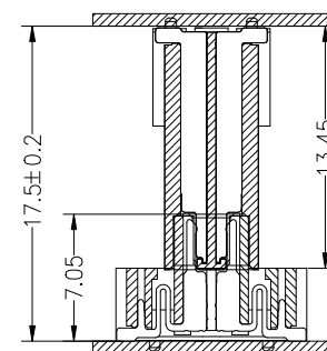
Mating Draw (Ref)
