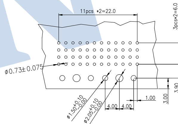
Recommended P.C.B Layout(Top Side) (PCB BOARD TOLERANCE±0.05)
